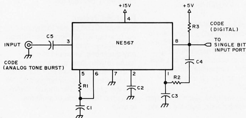
Figure 6: A suggested selective input filter for better performance. This circuit is adapted from the Signetics Catalog, page 6-97. The design equations are shown. The phase lock loop "latches up" when the signal is detected in the filter's band, typically after several tens of cycles. C3 determines the time taken for the filter to detect this condition. The time taken to unlatch after the signal disappears is determined by R2 and C4, with some effects from C3.
